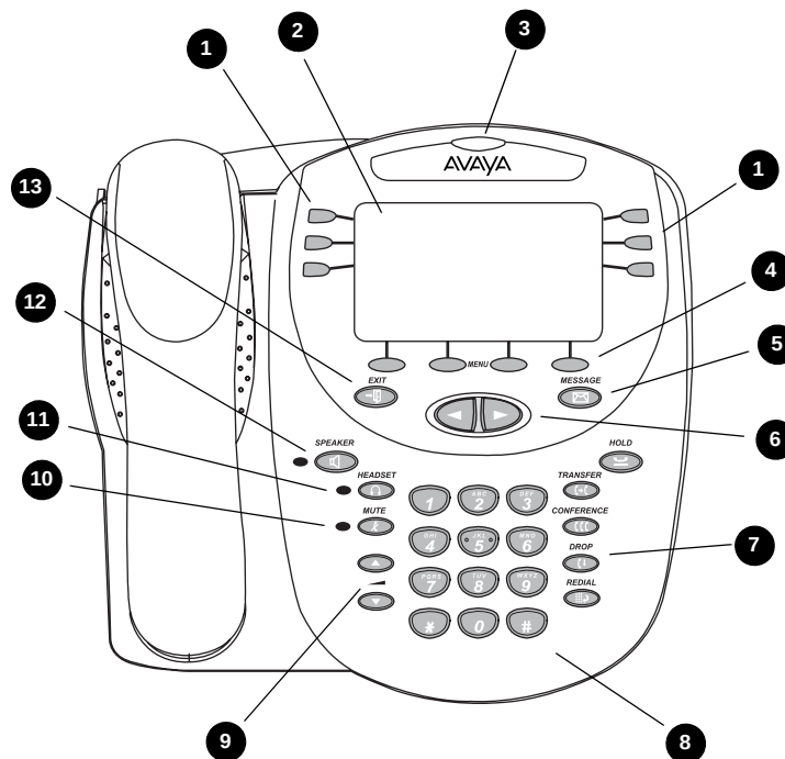
Figure 1: 2410 Telephone Components
