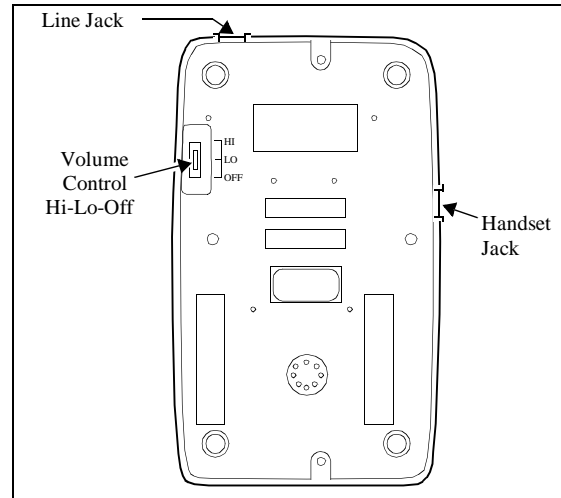
The 2500 MMGN and 2500 YMGP, Bottom View
