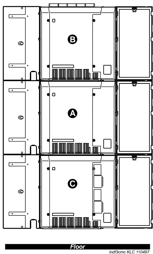
Figure 46: Typical vertical installation, front view of the CMC1 Media Gateway, DEFINITY Server CSI configuration
