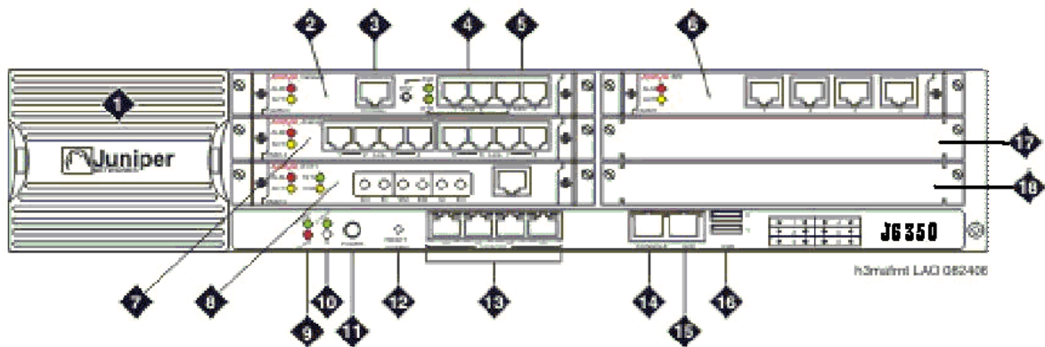
Figure 32: The IG550 Integrated Gateway in a J6350 Services Router
