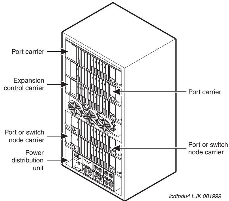
Figure 54: MCC1 EPN or PN cabinet
