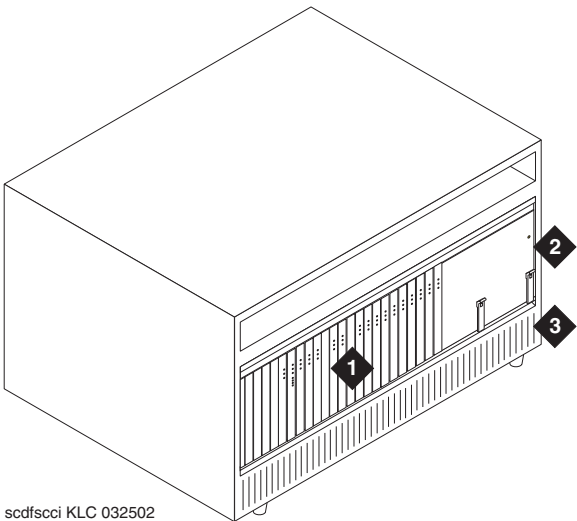
Figure 47: Typical SCC1 Media Gateway
