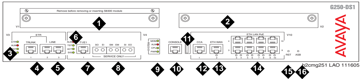
Figure 28: The Avaya G250-DS1 Media Gateway Chassis
