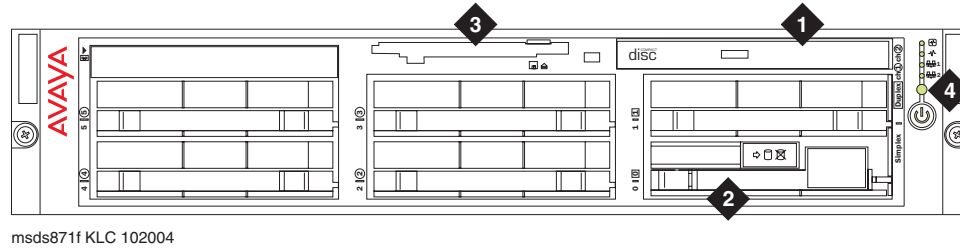
Figure 16: S8710 Media Server (front view)
