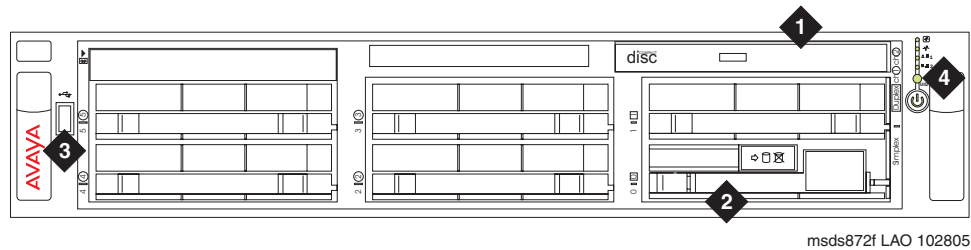
Figure 13: S8720 Media Server (front view)
