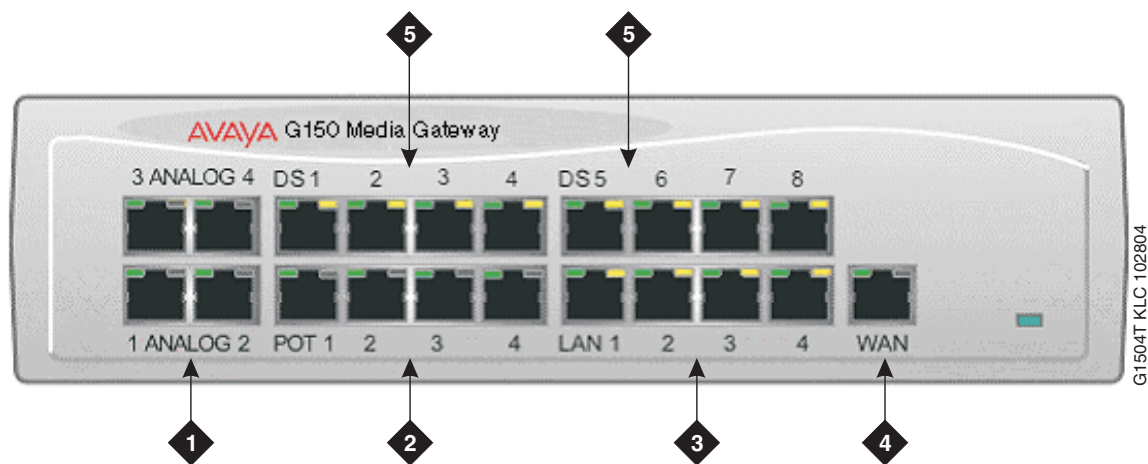
Figure 22: G150 4T+4A (16 VoIP) Front Panel
