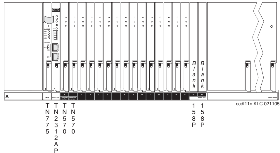
Figure 51: Expansion control cabinet (J58890N)
