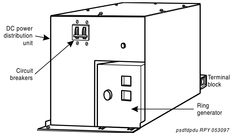
Figure 91: DC power-distribution unit (J58890CF-2) (front view))
