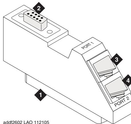
Figure 63: IP Media Resource 320 I/O adapter
