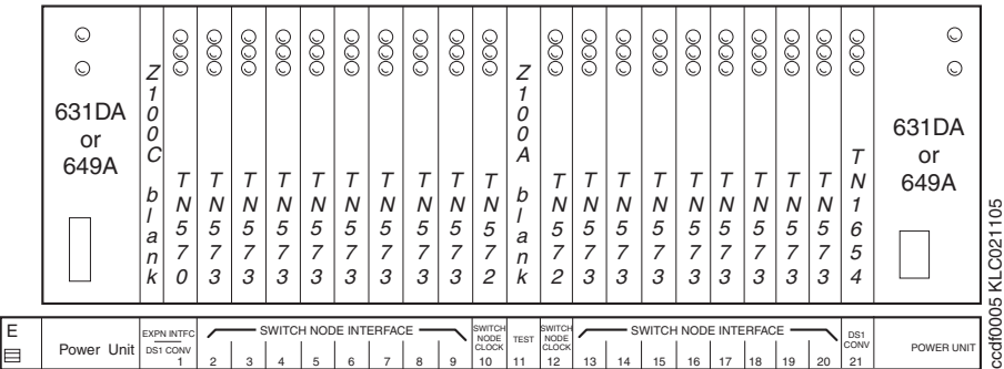
Figure 58: Switch node carrier (J58890SA)
