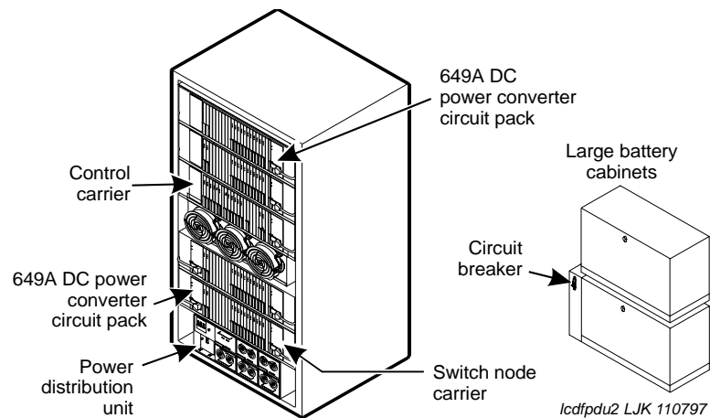
Figure 93: DC power distribution in MCC1s
