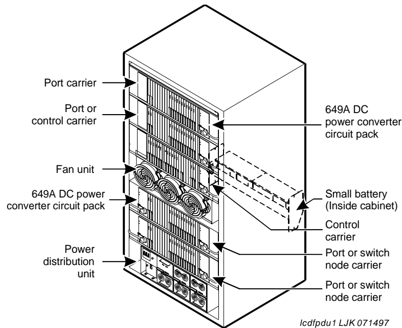
Figure 92: Power distribution in MCC1
