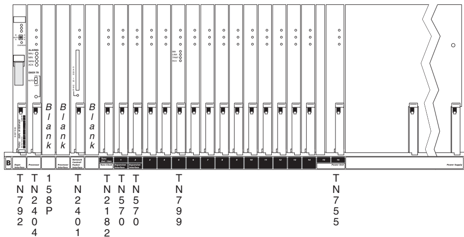
Figure 50: Duplicated control cabinet (J58890M)
