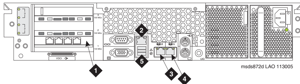
Figure 15: S8720 Media Server (back view) with software duplication
