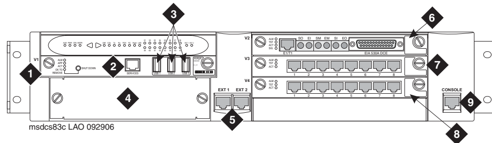
Figure 1: S8300 Media Server in a G700 Media Gateway (S8300C shown)
