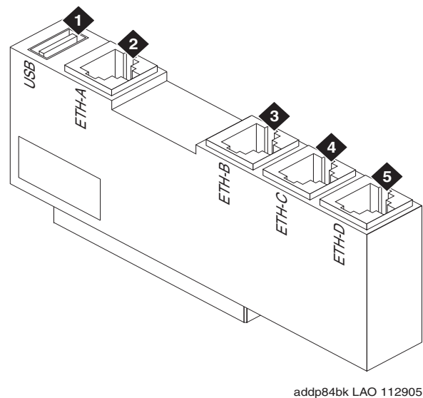
Figure 6: Media server cable adapter
