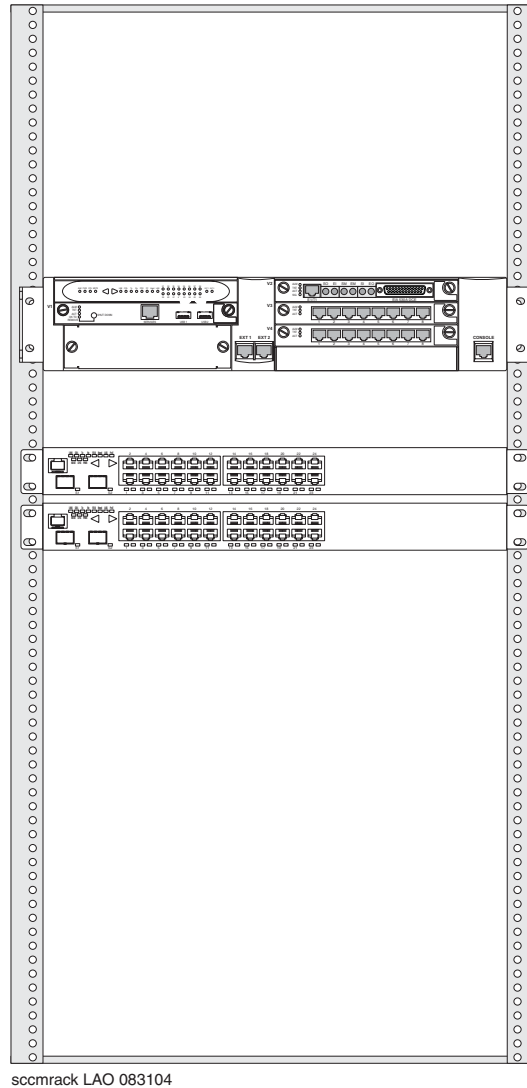
Figure 36: G700 Media Gateway with two Avaya C360 switches
