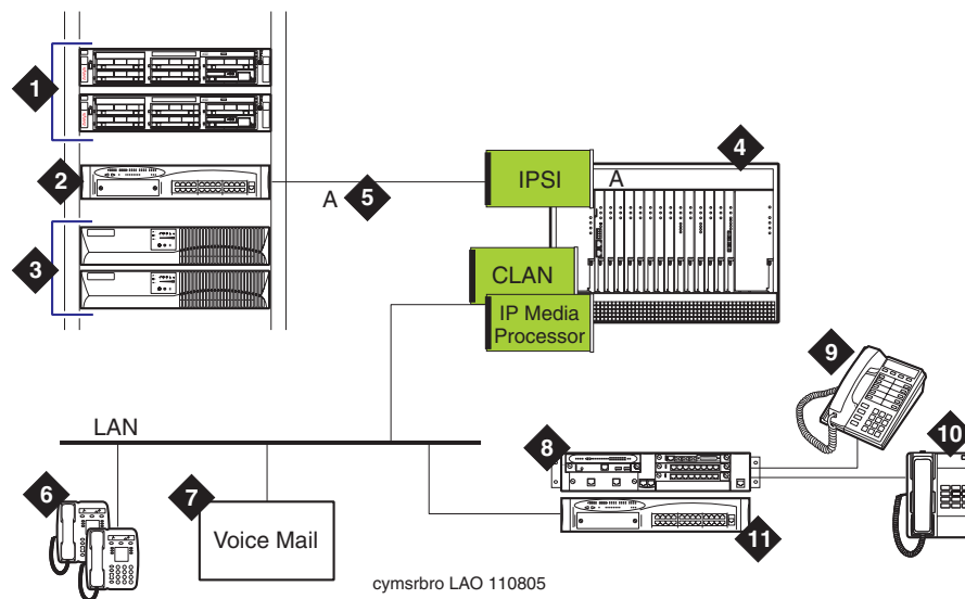
Figure 37: The G700 Media Gateway connecting to the S8700-series Media Server
