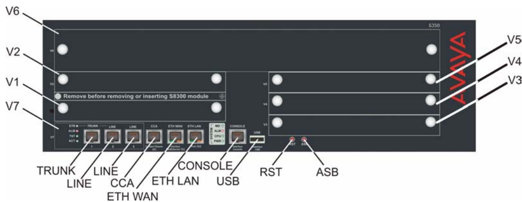
Figure 29: G350 chassis
