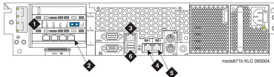
Figure 17: S8710 Media Server (back view)
