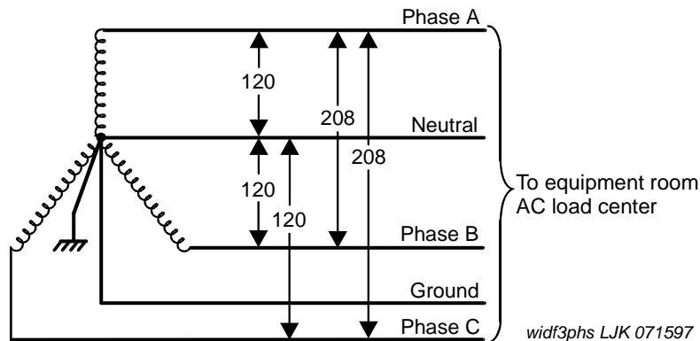
Figure 82: 3-phase, 120- to 208-VAC, 60-Hz source
