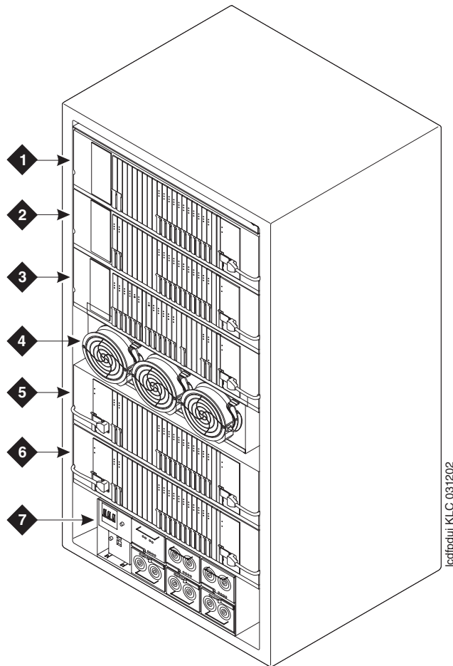
Figure 53: Typical PN cabinet for all server models
