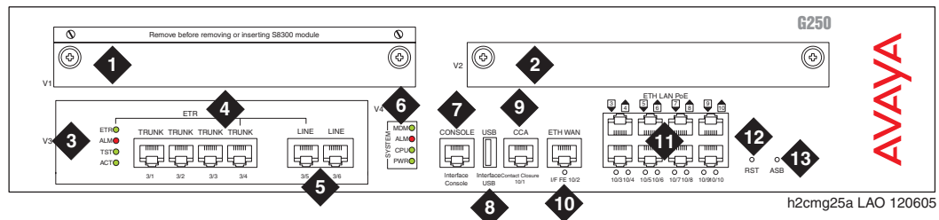
Figure 25: The Avaya G250-Analog Media Gateway Chassis
