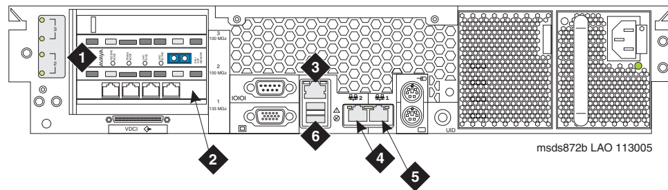
Figure 14: S8720 Media Server (back view) with hardware duplication
