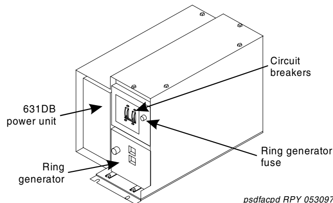
Figure 85: AC power-distribution unit (J58890CE-2) (front)
