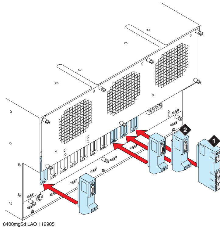
Figure 8: TN8412AP and TN8400AP backplane connectors on a G600 Media Gateway
