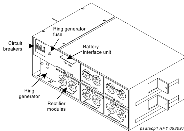
Figure 88: AC power-distribution unit (J58890CH-1) (front)
