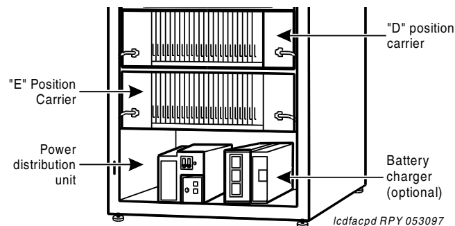
Figure 87: AC power distribution in MCC1 cabinets
