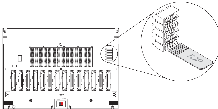
Figure 42: Printed circuit card
