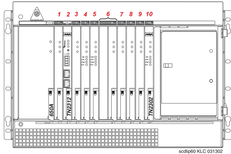
Figure 40: G600 Media Gateway
