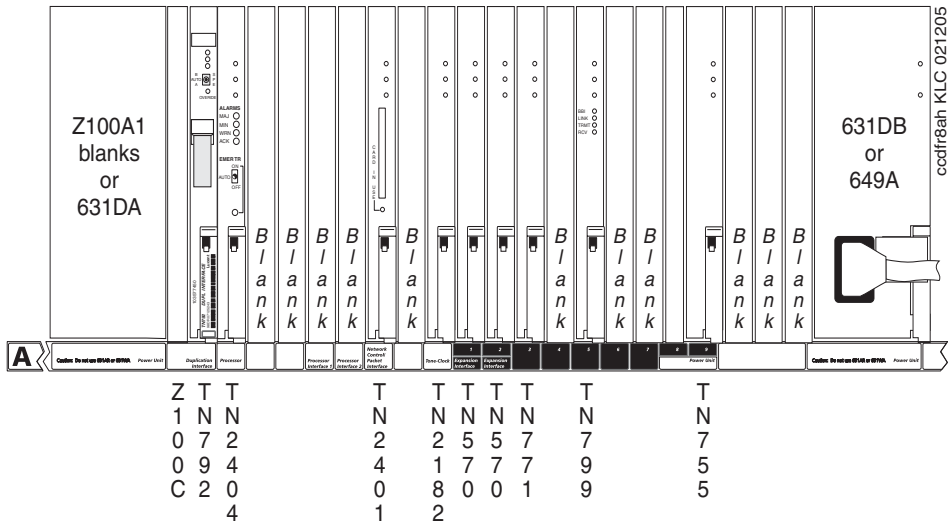
Figure 55: Control carrier (J58890AH)
