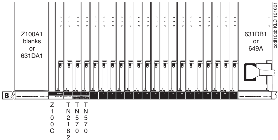
Figure 57: Port carrier (J58890BB)
