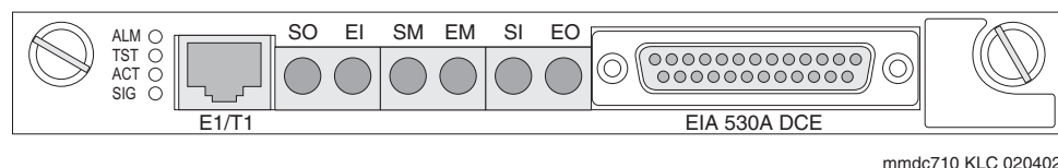
Figure 65: Avaya MM710 T1/E1 Media Module
