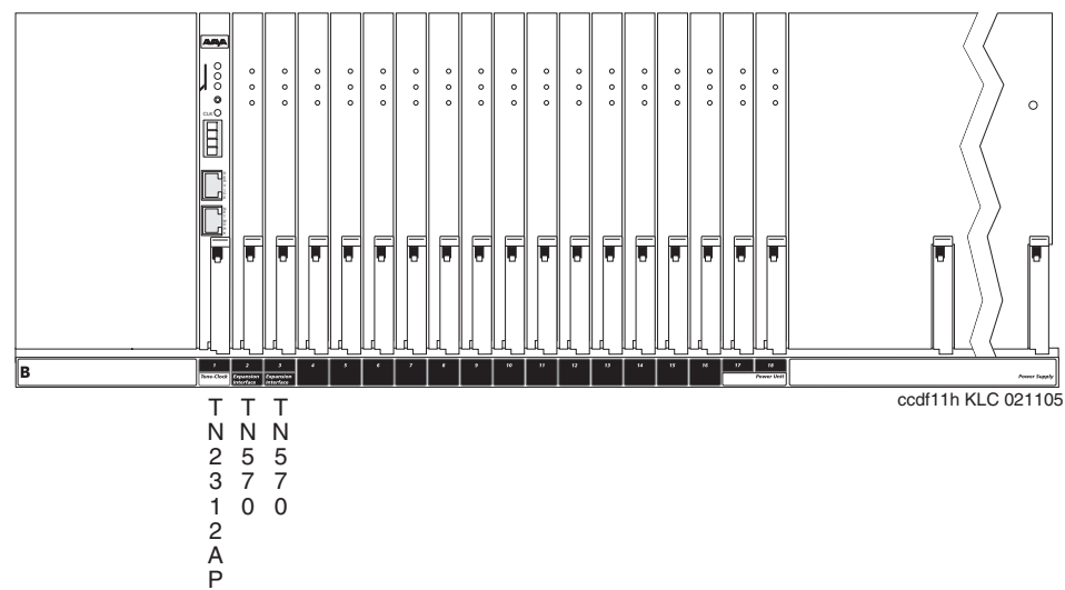
Figure 52: Port cabinet (J58890H)
