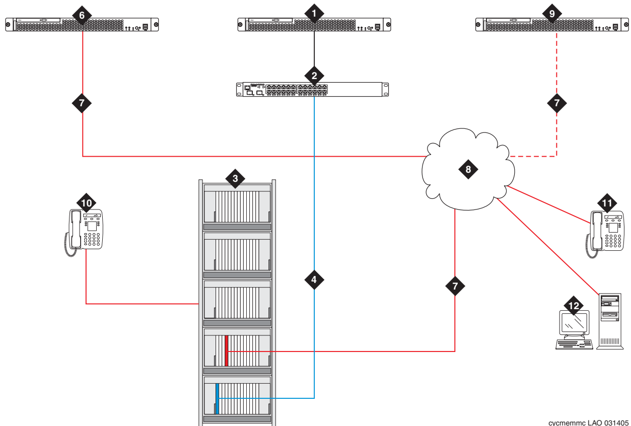
Figure notes: EMMC architecture (example with an S8500 Media Server for Communication Manager)
