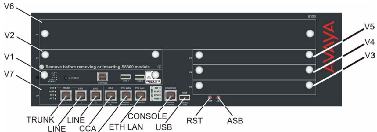
Figure 2: S8300 Media Server in a G350 Media Gateway (S8300B shown)
