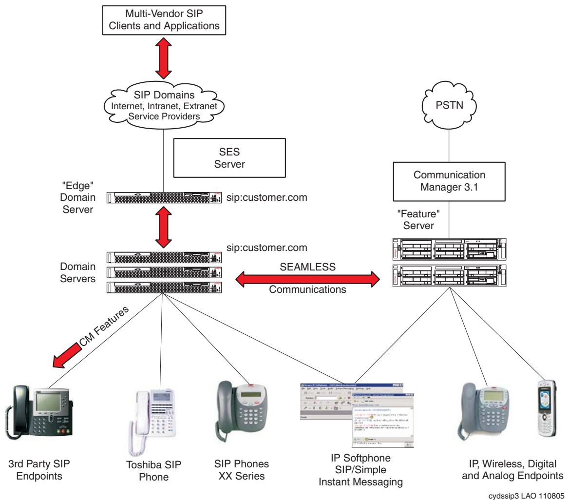
Figure 18: SIP Architecture
