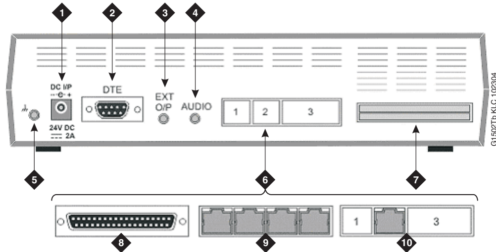
Figure 23: G150 4T+4A (16 VoIP) Back Panel
