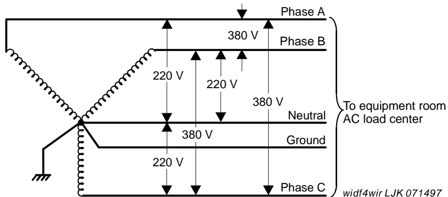
Figure 83: International, 3-phase, 220- to 380-VAC, 50-Hz source
