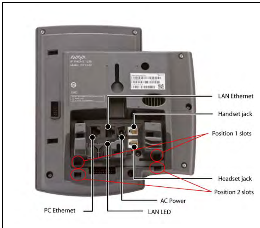
Figure 8: IP Deskphone connections
