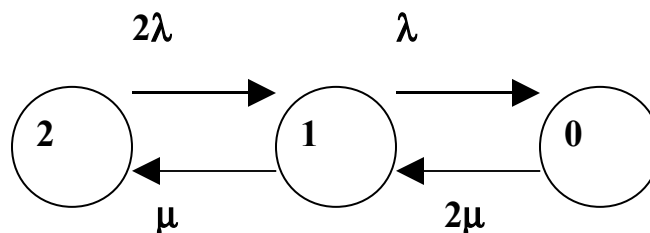
Figure 8: State Transition Diagram for Redundant Components
