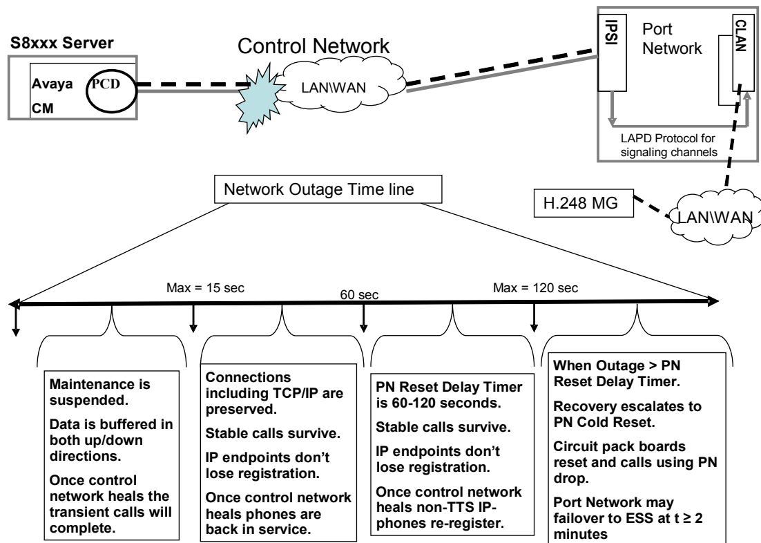
Figure 5: Improved Port Network (PN) Recovery from Control Network Outages
