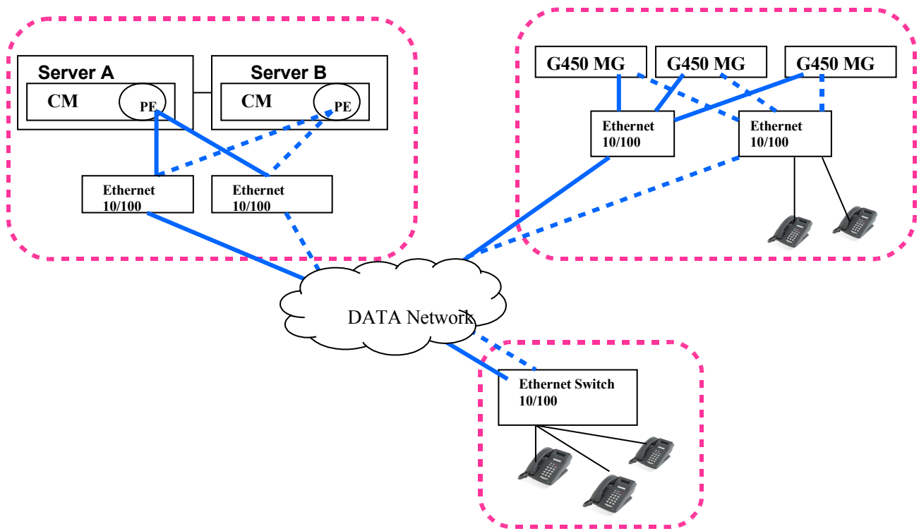
Figure 3: S8800 Server Pair Support Remote IP-phones and H.248 Media Gateways on Processor Ethernet for Duplex Servers
