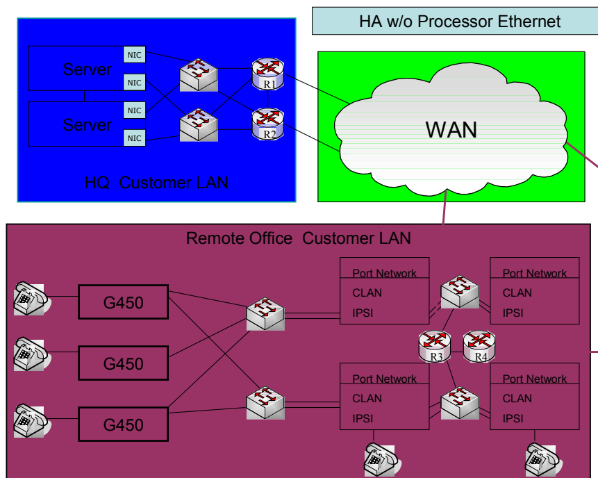
Figure 6: Example of a Network Designed for High Availability at the Remote Office
