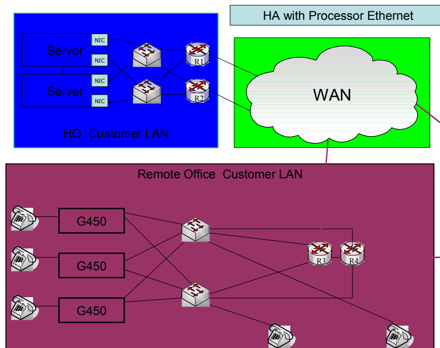
Figure 7: Example of a Network Designed for High Availability with Processor Ethernet
