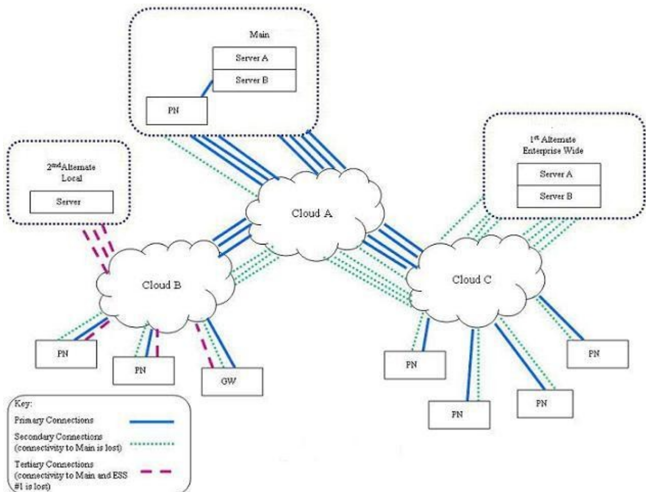
Figure 4: Example of Cluster of Survivable Servers both at Enterprise Level and Local Level
