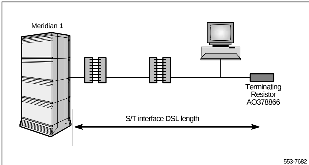
Figure 20 Point-to-point DSL
