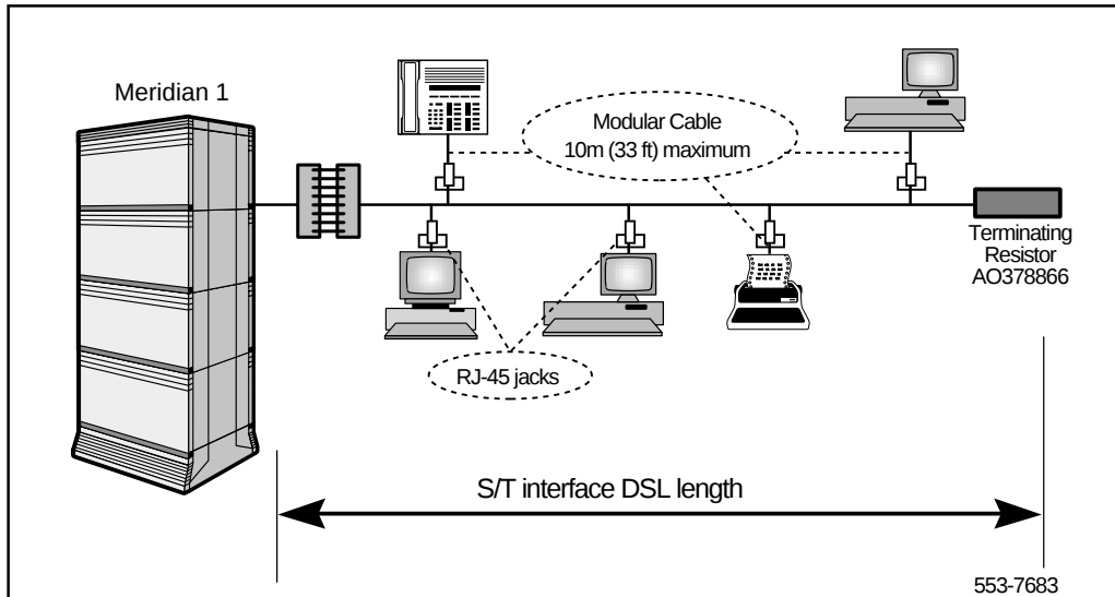
Figure 21 Short passive SILC DSL
