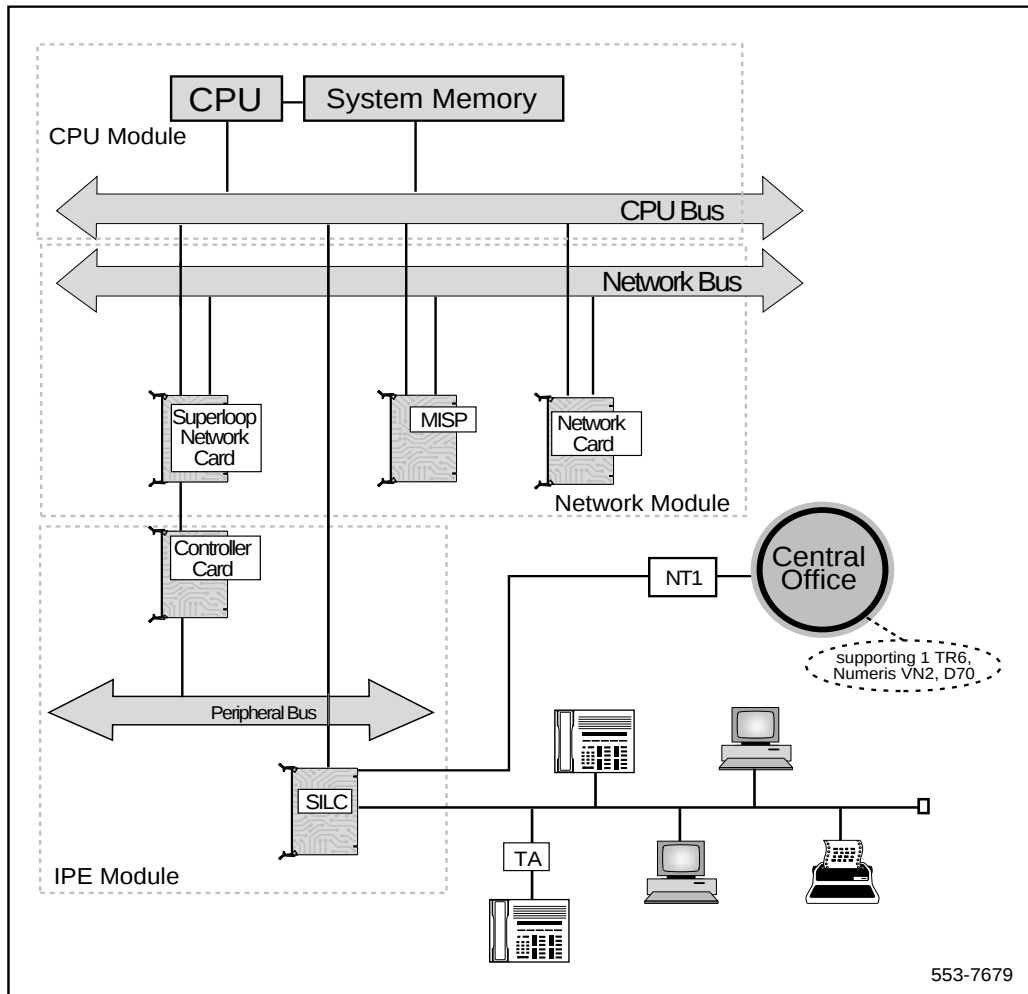
Figure 17 A basis ISDN BRI trunking architecture (CO connectivity)
