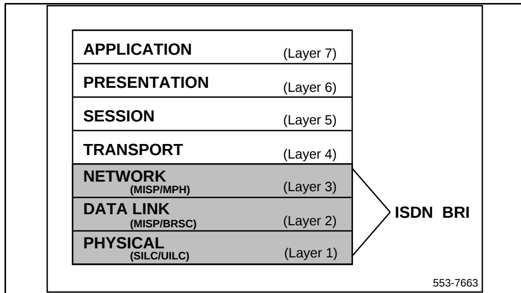
Figure 1 OSI model
