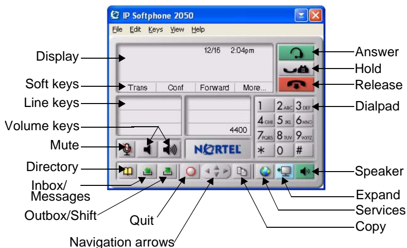
Figure 4: Call Control Window—Compact Theme (silver)
