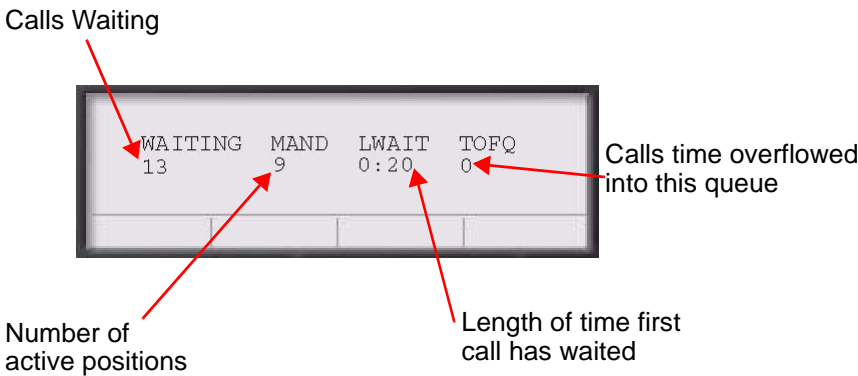
Figure 9: Display Queue
