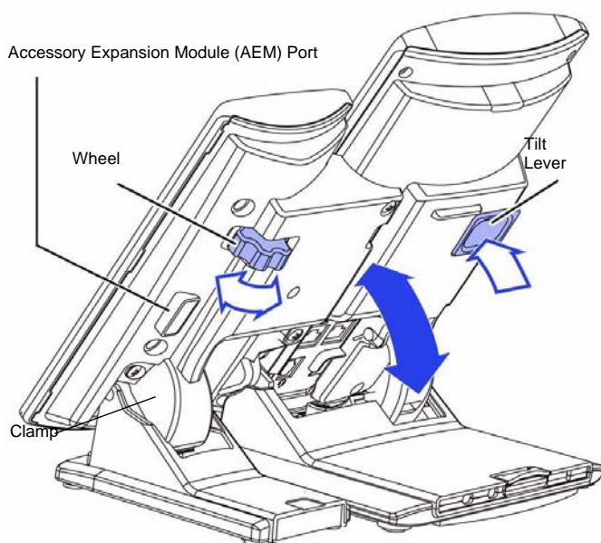
Figure 3: Adjusting the stand angle on the IP Deskphone
