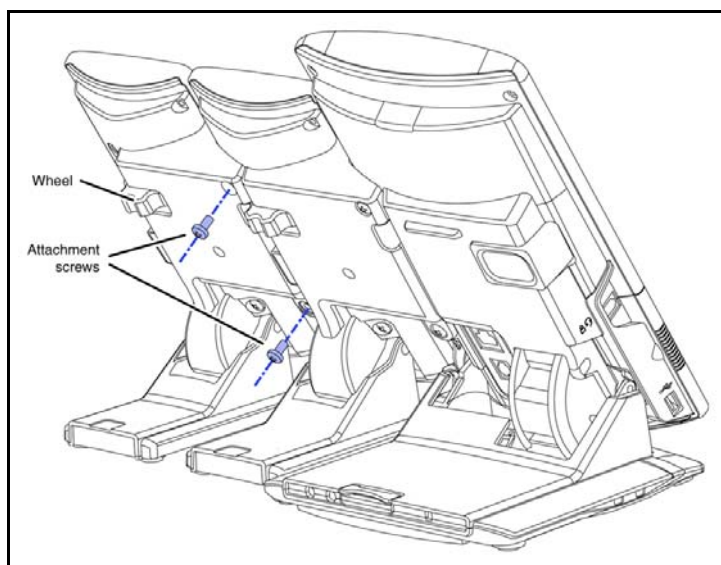
Figure 4: Connecting the Expansion Module
