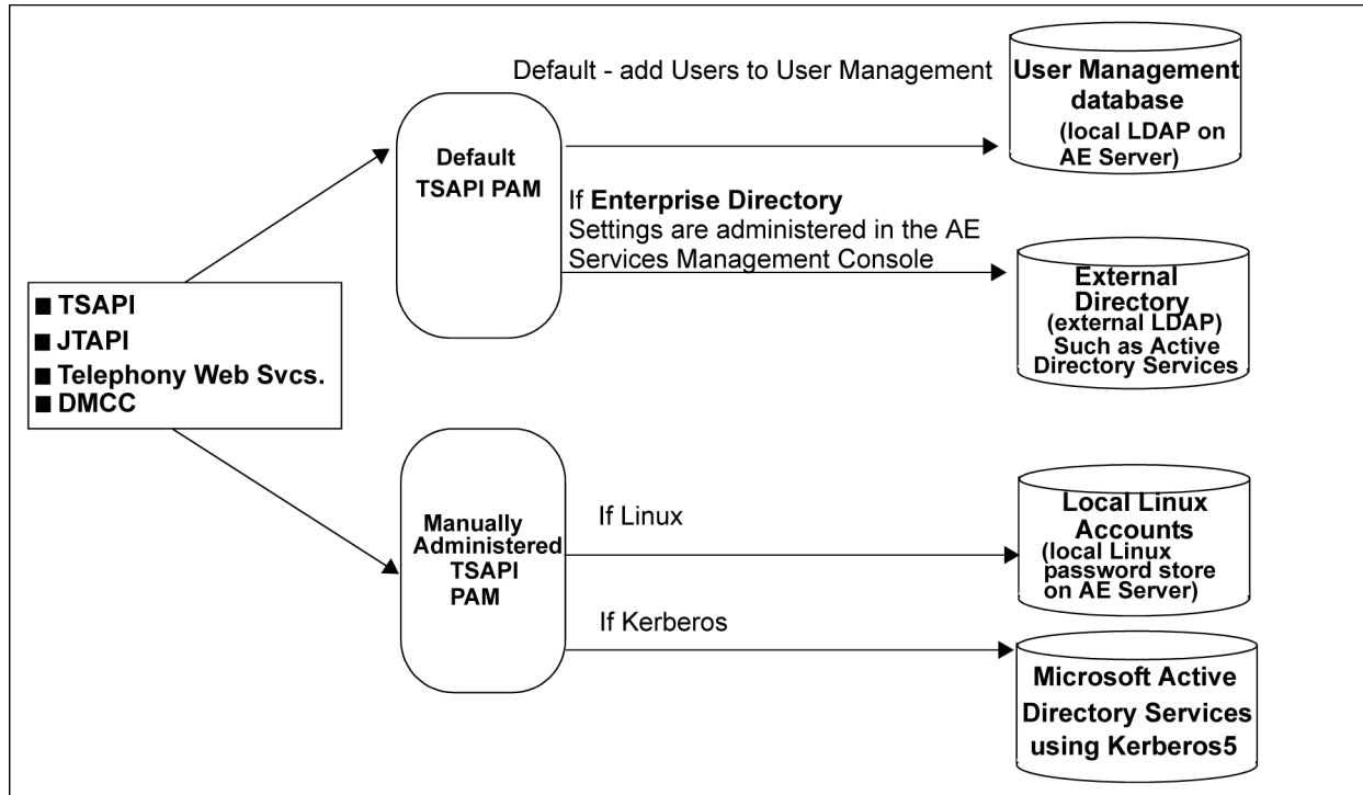
Figure 28: AE Services client authentication -- additional PAM management
