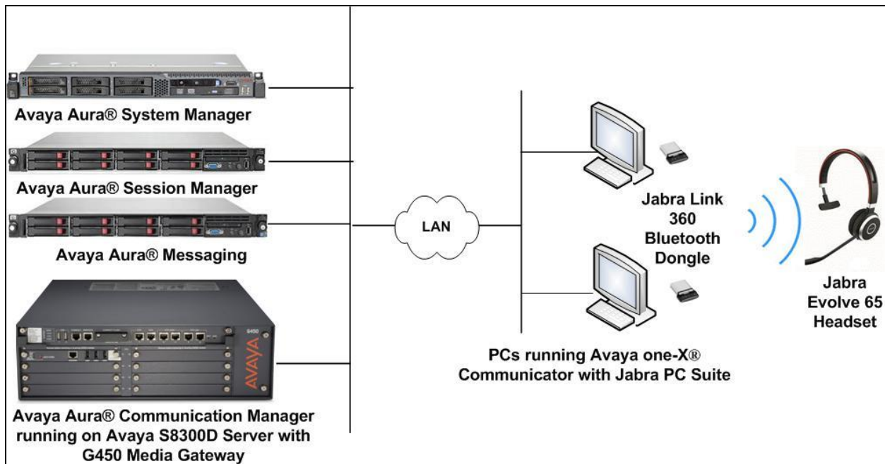
Figure 1: Test Configuration
