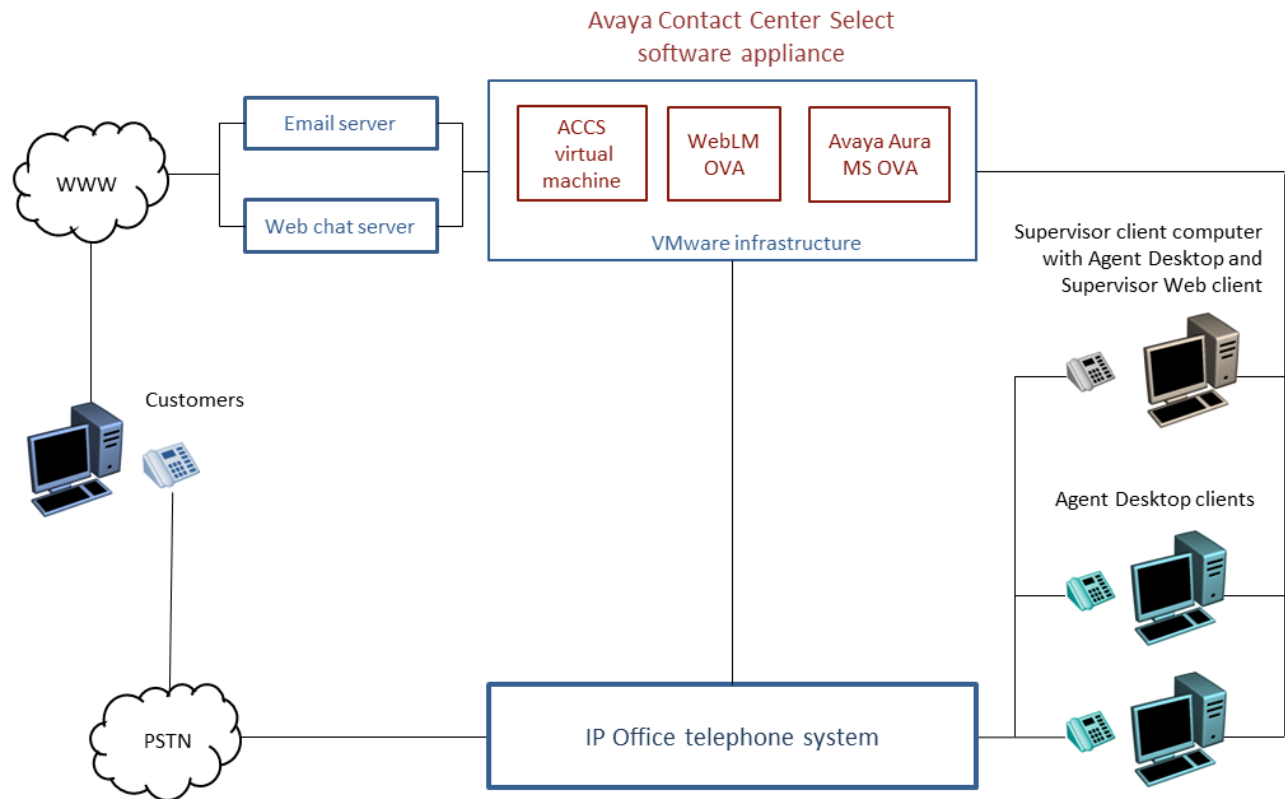
Figure 9: Typical virtualized contact center solution using Avaya Contact Center Select, Avaya Aura® Media Server, and Avaya WebLM deployed on a single VMware host server
