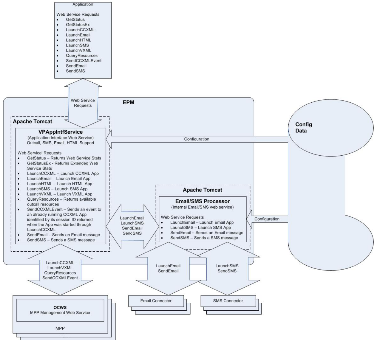
Figure 1: Application Interface Web service flow diagram
