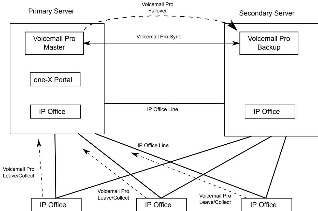
Figure 10: One active Voicemail Pro server
