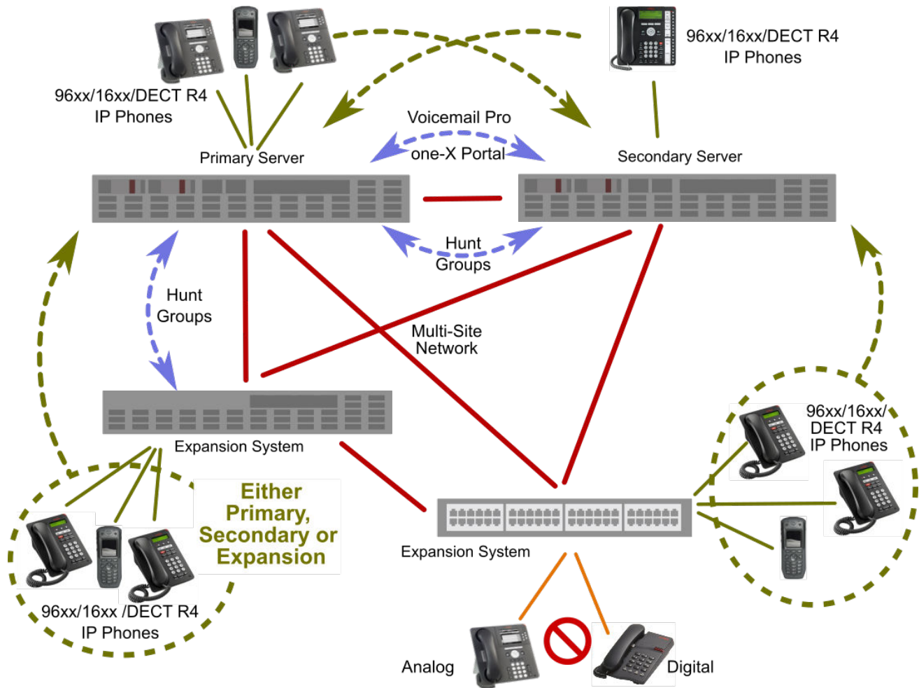
Figure 9: Resiliency Architecture
