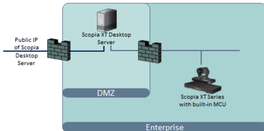
Figure 4: Scopia XT Desktop with a dual-NIC deployment
