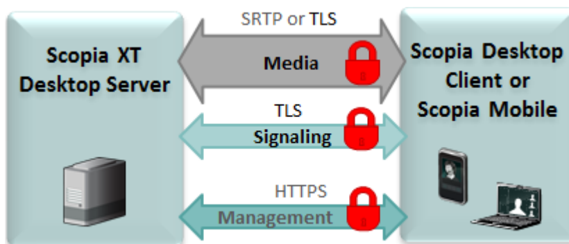
Figure 44: Encrypting communications using TLS
