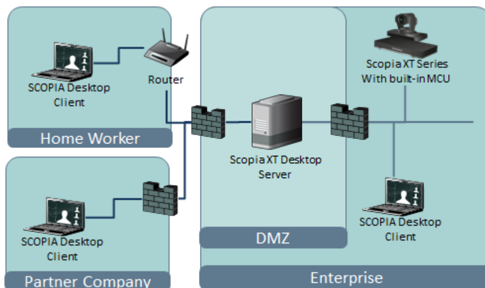
Figure 5: Locating the Scopia XT Desktop Server in the DMZ
