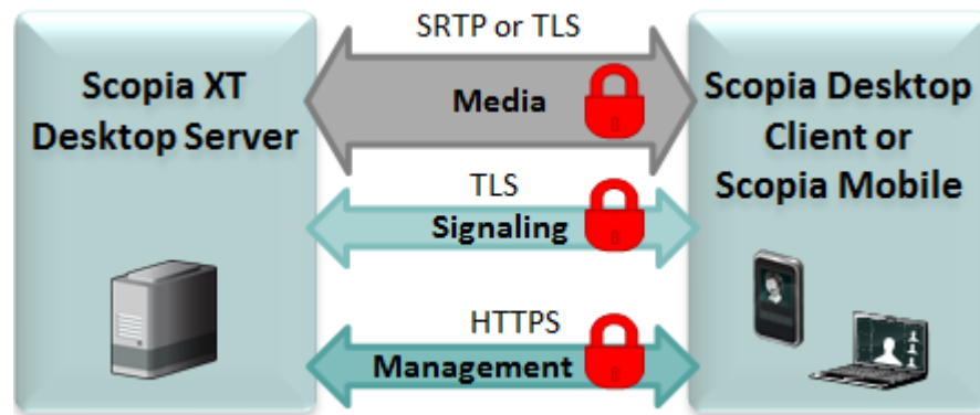
Figure 40: Encrypting communications between Scopia XT Desktop Server and Scopia XT Desktop Client
