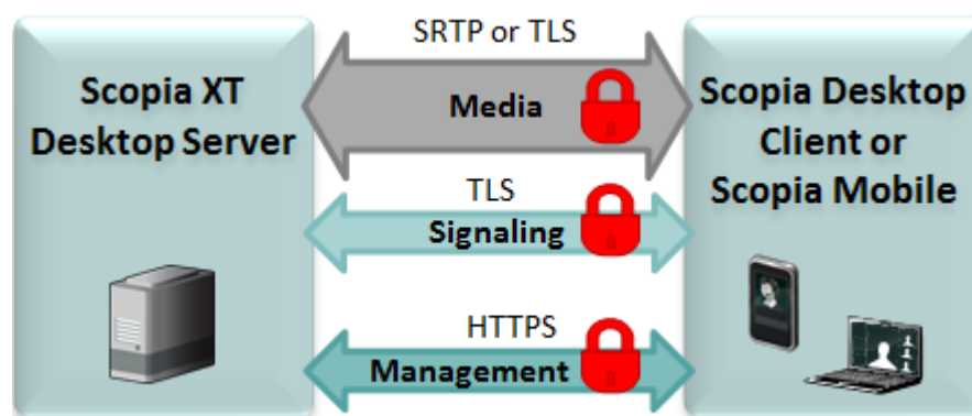
Figure 39: Protocols used in a secure environment
