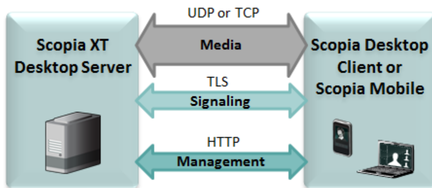
Figure 38: Protocols used in an unsecure environment
