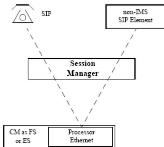
Figure 33: Call between a SIP station and a non-IMS SIP element
