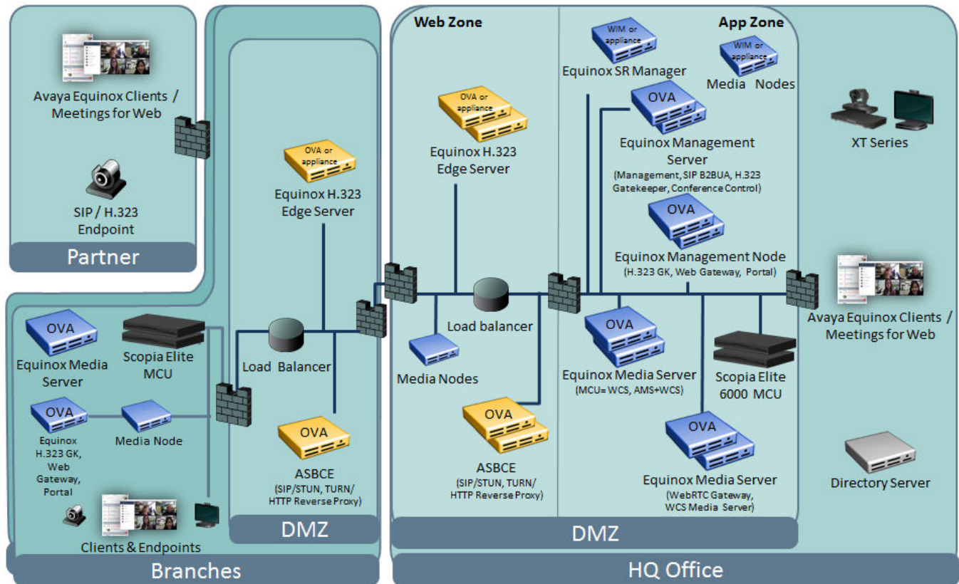
Figure 3: OTT Large Distributed configuration
