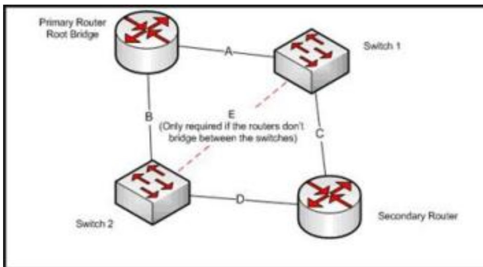
Figure 20: Sample spanning tree
