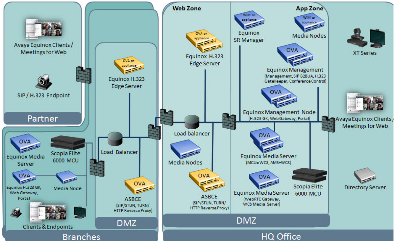
Figure 6: OTT deployment for medium to large enterprises
