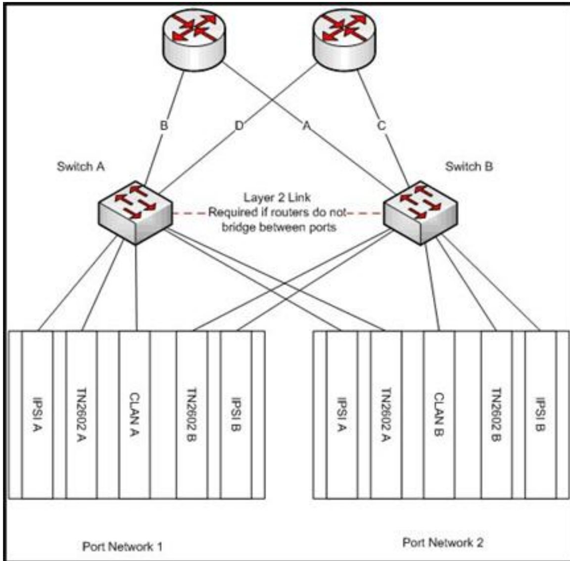
Figure 19: Redundant connections
