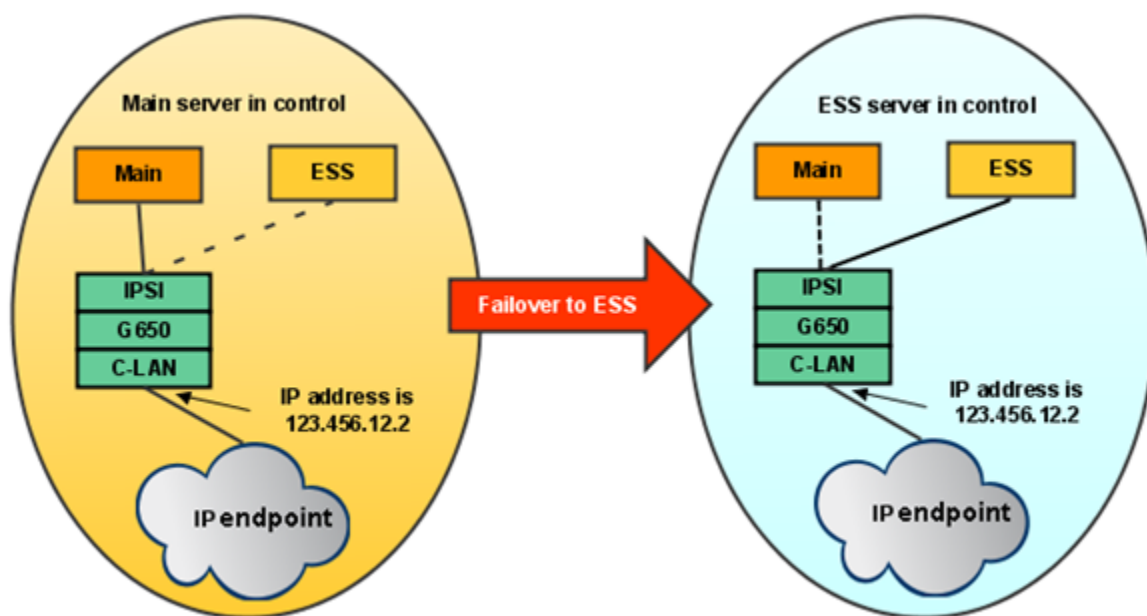
Figure 11: IP device with C-LAN
