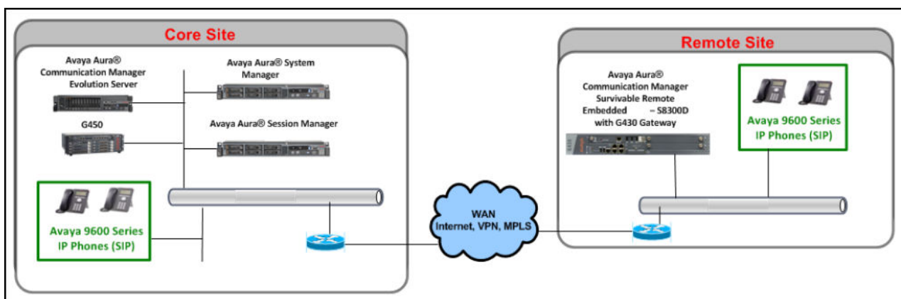
Figure 9: Avaya Aura® with Embedded Survivable Remote
