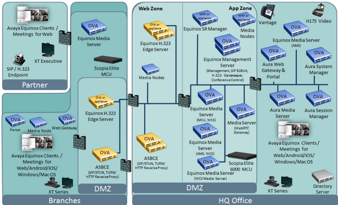
Figure 4: TE UC Distributed configuration
