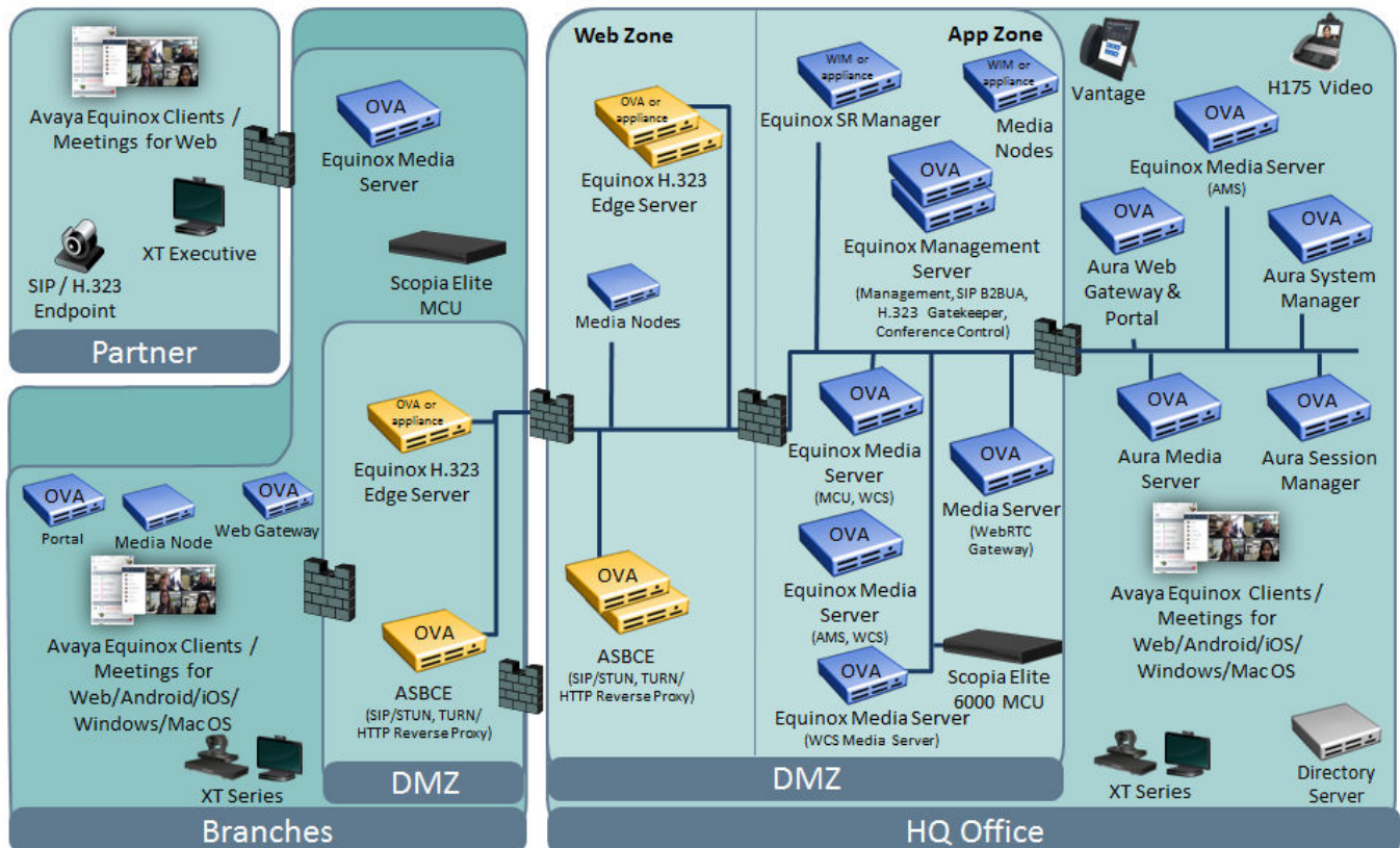
Figure 7: TE deployment for medium to large enterprises
