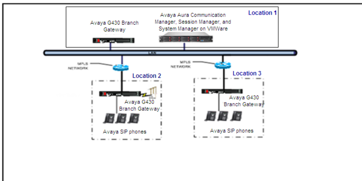
Figure 10: Avaya Aura® on VMware
