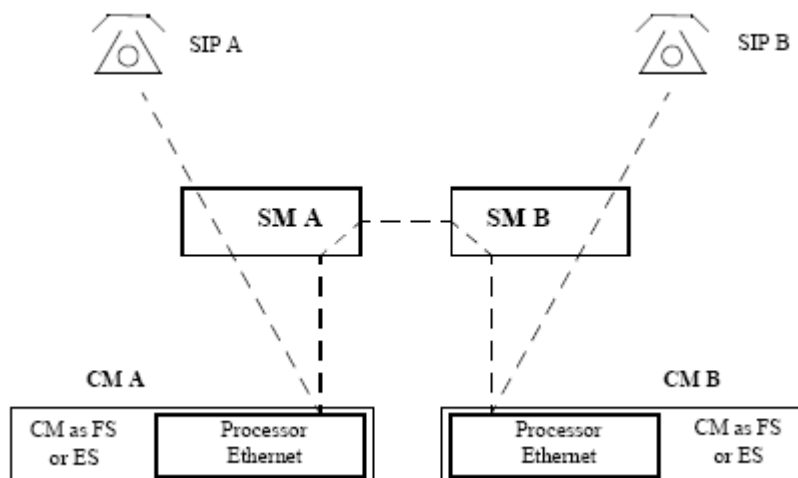
Figure 32: Call between two SIP stations with different Session Manager instances and different Communication Managers
