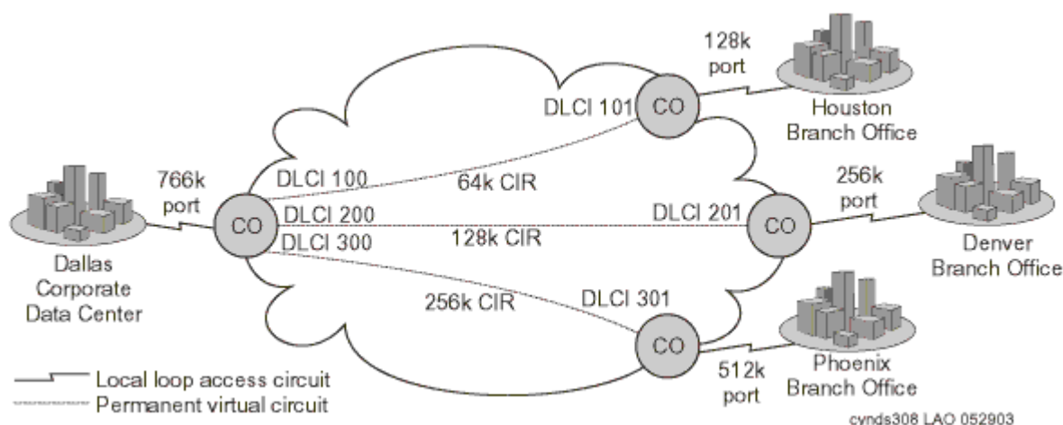
Figure 14: Data-link connection identifiers over an interexchange carrier Frame Relay network
