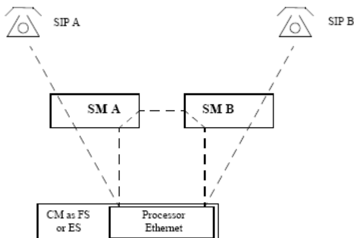
Figure 31: Call between two SIP stations with different Session Manager instances and same Communication Manager
