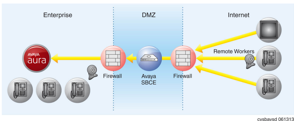
Figure 27: Advanced Services Solution
