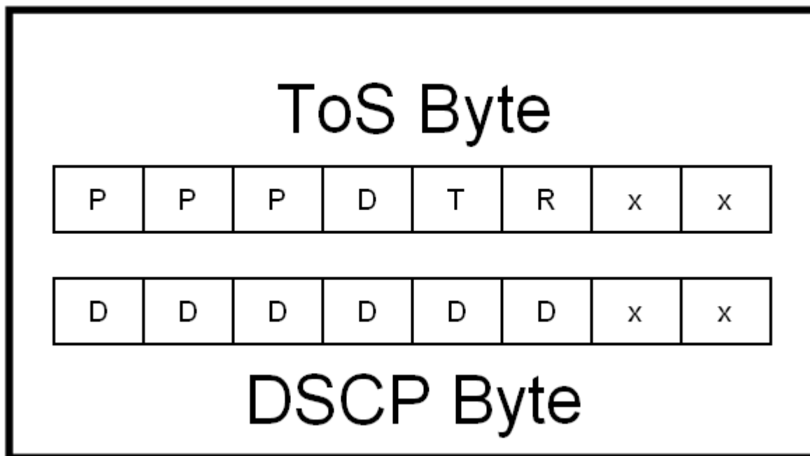
Figure 23: Comparison of DSCP with original ToS
