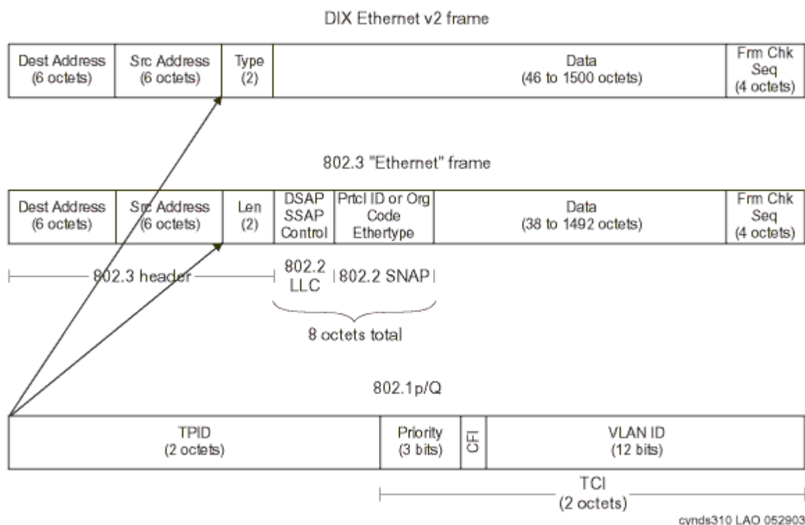
Figure 24: 802.1Q tag
