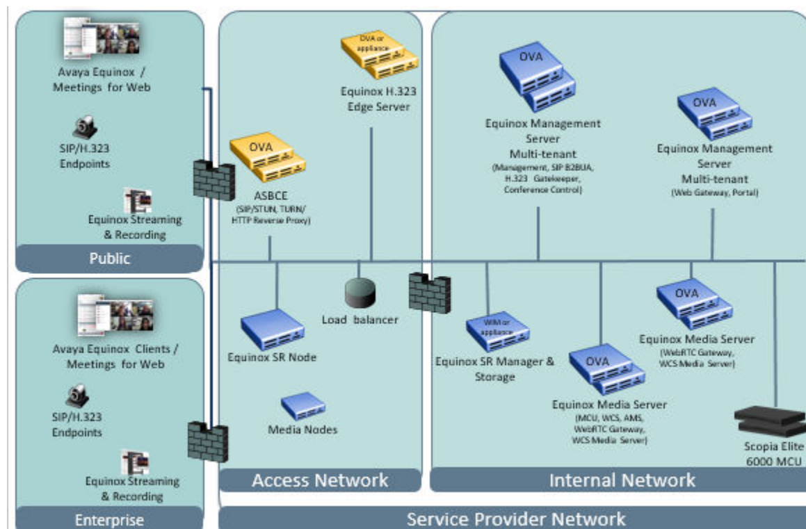
Figure 5: OTT Configuration for Service Providers and Cloud services
