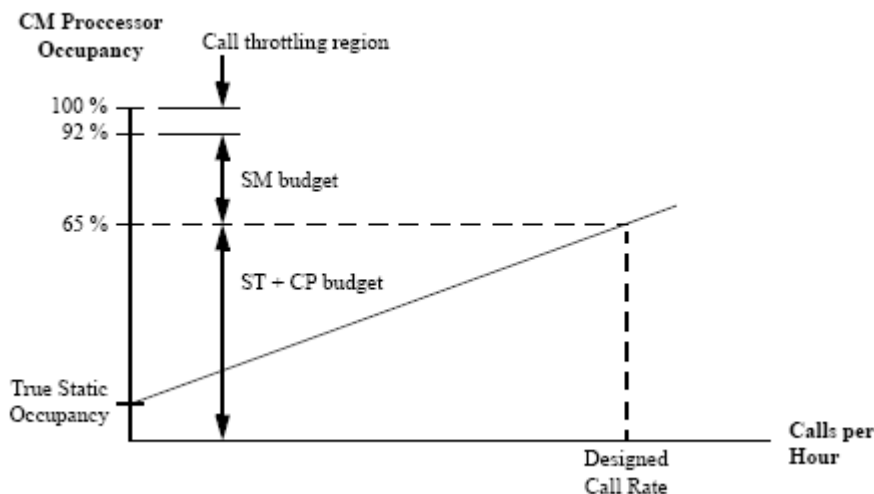
Figure 38: Processing occupancy budgets for Communication Manager
