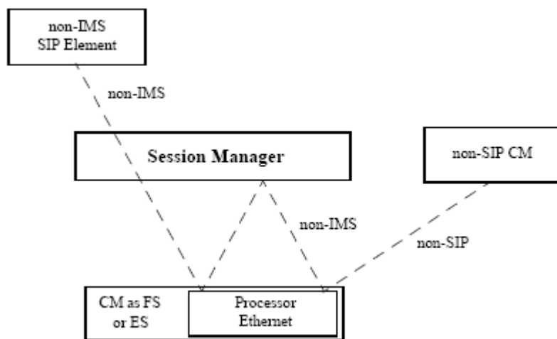
Figure 36: Call between a non-IMS SIP element and a non-SIP Communication Manager
