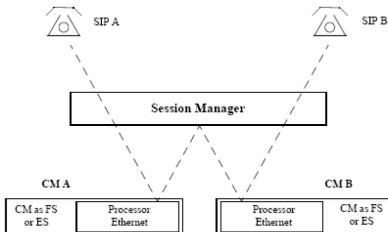
Figure 30: Call between two SIP stations with same Session Manager instance and different Communication Managers
