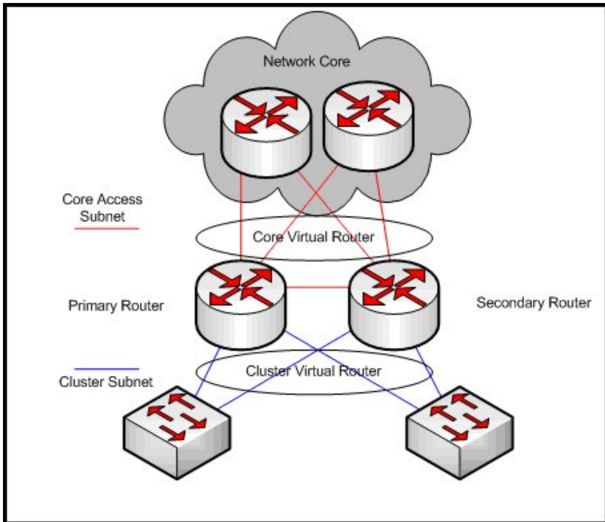
Figure 22: VRRP configured for Core Access
