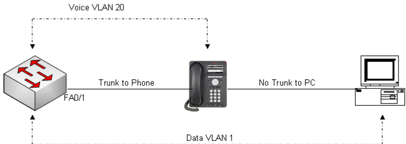
Figure 13: Trunking for softphones or physical phones
