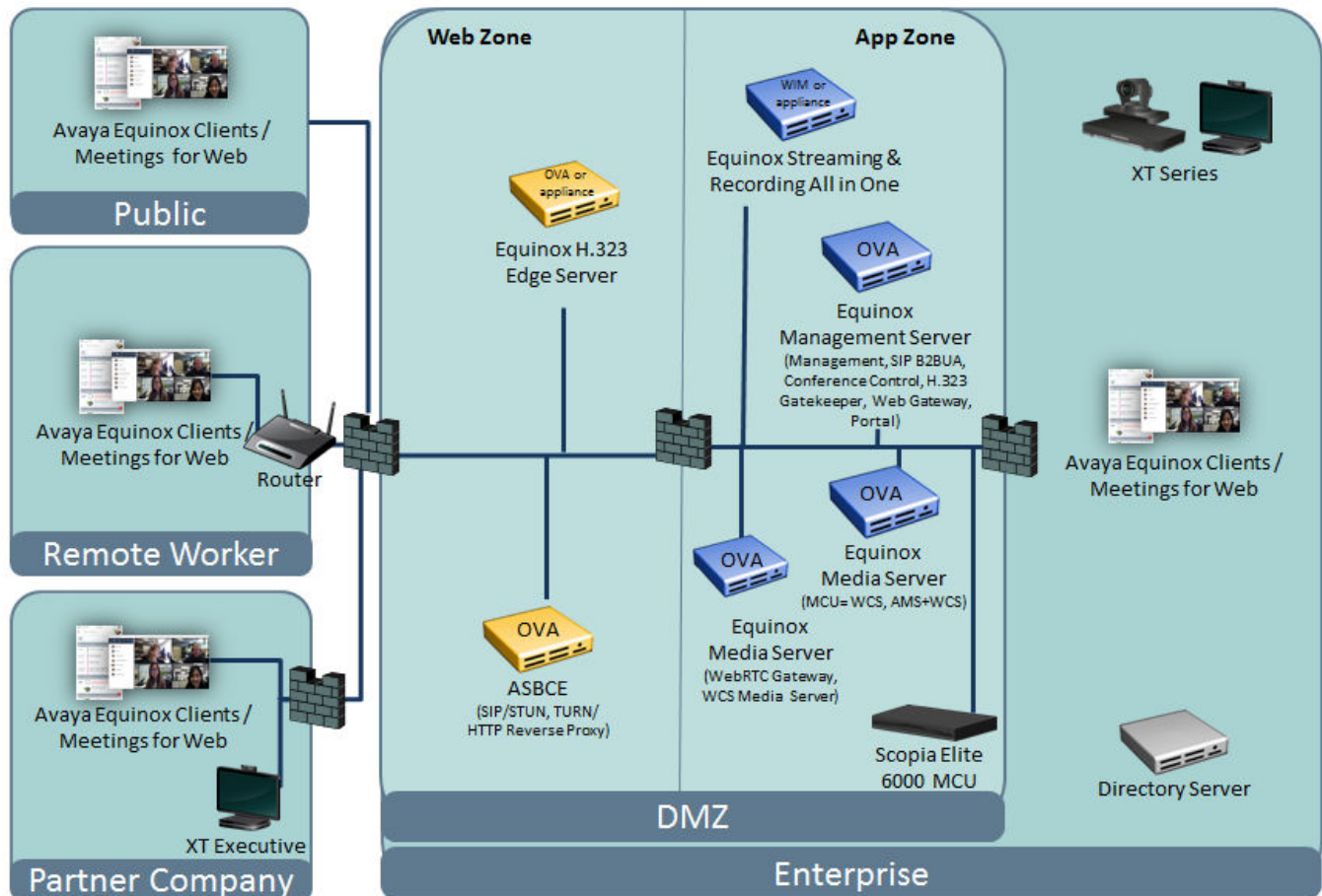
Figure 8: Example of a complete centralized solution
