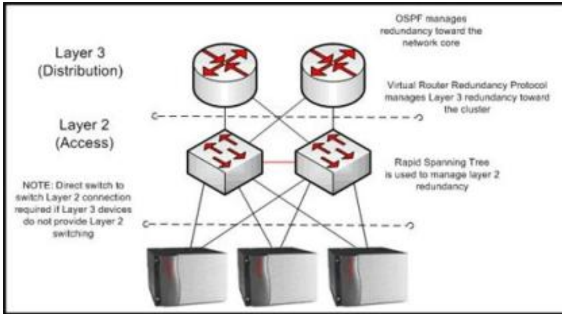
Figure 18: Layered Server Cluster Topology
