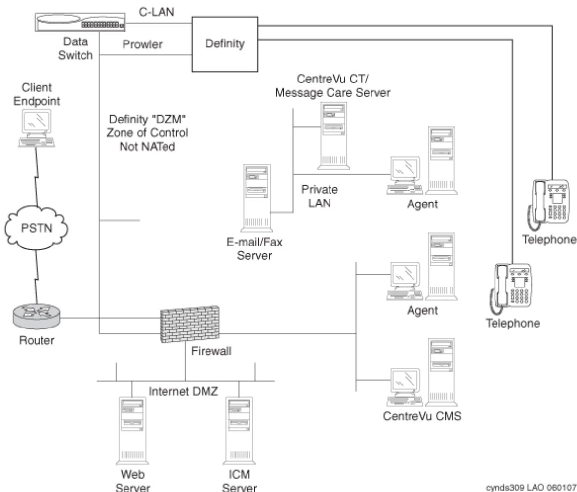
Figure 16: IP telephony without NAT
