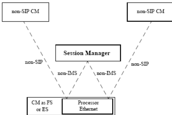
Figure 37: Call between two non-SIP Communication Managers
