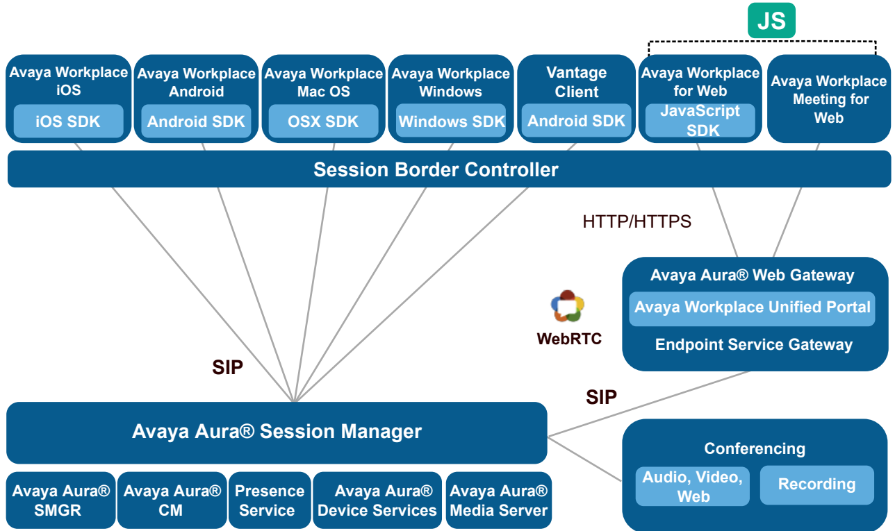
Figure 1: Avaya Workplace Client and Conferencing deployment topology
