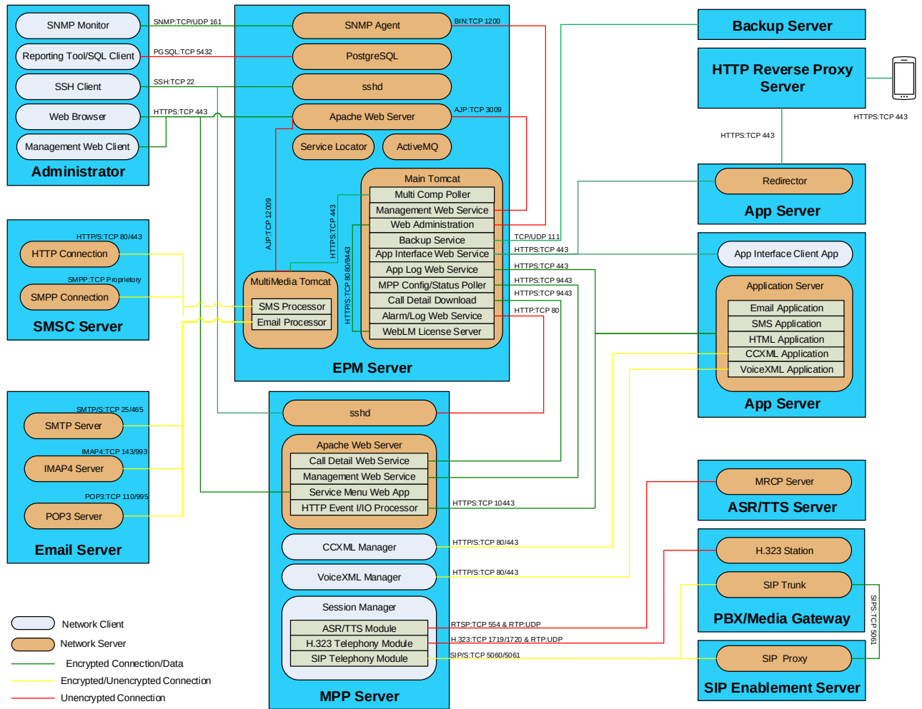
Figure 1: Network services & clients required for operation of the Experience Portal
