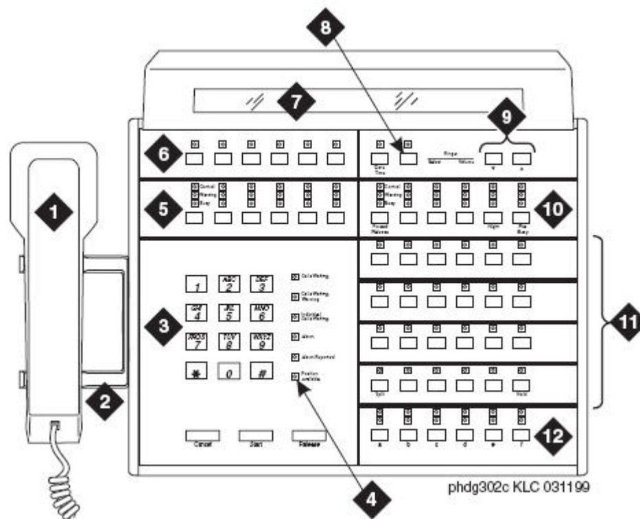
Figure 2: 302C attendant console
