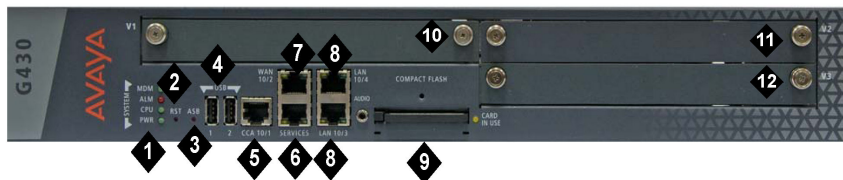
Figure 1: G430 Branch Gateway Chassis
