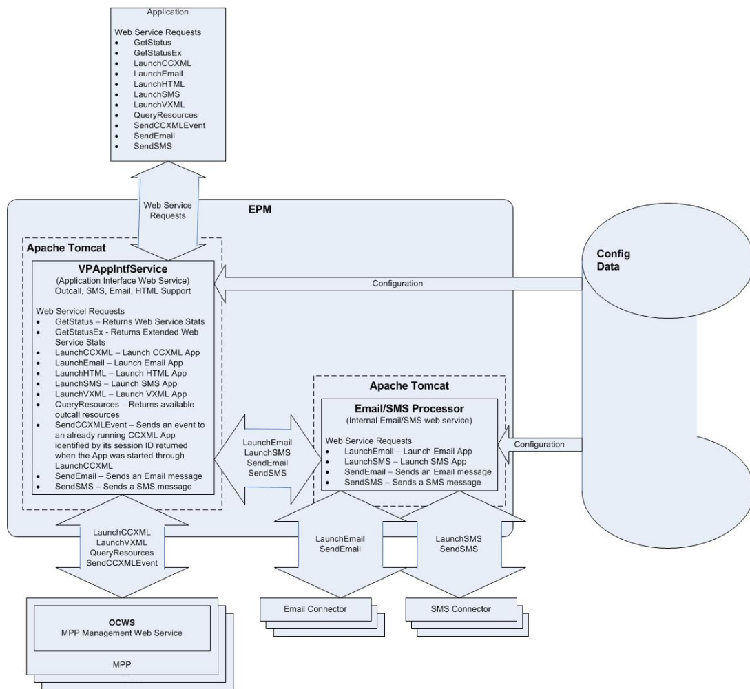
Figure 1: Application Interface Web service flow diagram
